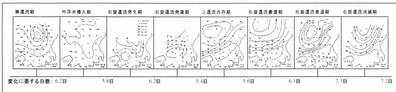
Fig.4 The examples of eight stages of flow patterns in Wakasa Bay (Hashimoto, 1982)
