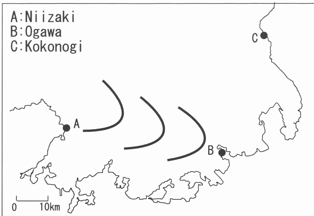
Fig.7 Schematic chart of a cold-water mass movement.
