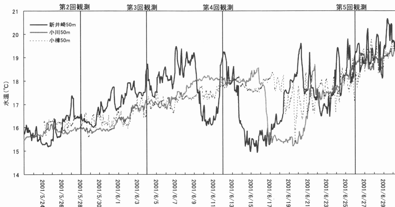
Fig.6 Time series of water temperature at moored stations.
